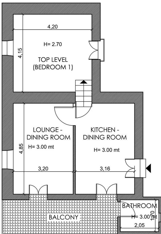
MIDDLE LEVEL (SHOWING STAIRS UP TO BEDROOM 1)
