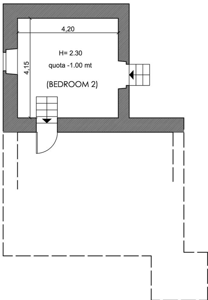
MIDDLE LEVEL (SHOWING STAIRS DOWN TO BEDROOM 2)
